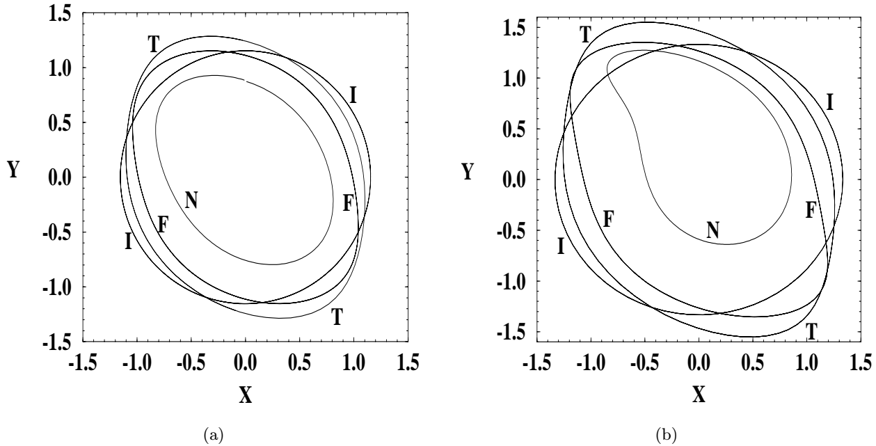
Fig. 1. Comparison of different approximations of periodic orbits for: (a) \mu = 0.3 ; (b) \mu = 0.4 . Label N corresponds to the exact orbit obtained by numerical integration. I indicates first-order approximation, T denotes the third-order approximation orbit and F corresponds to orbit obtained with the fifth-order approximation.
